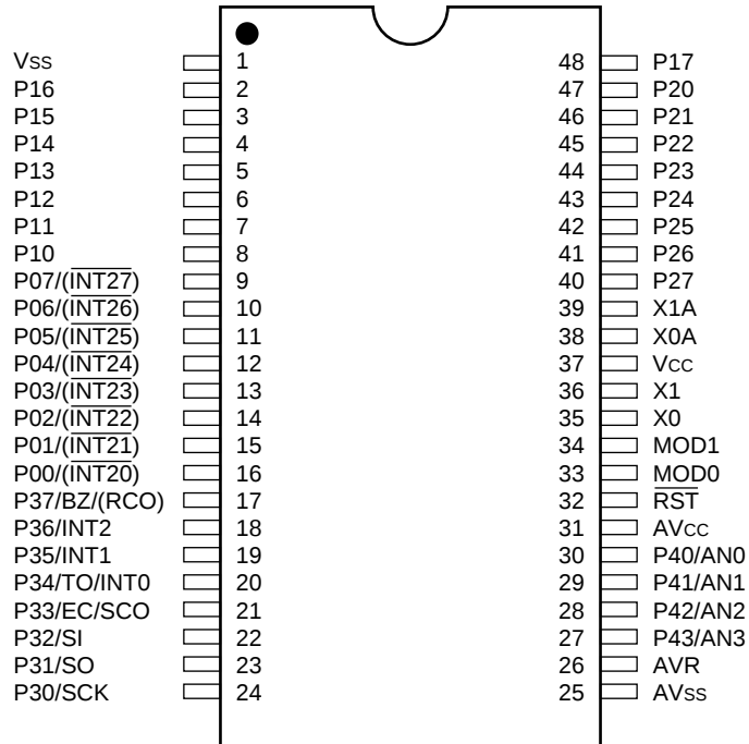
(DIP-48P-M01)
