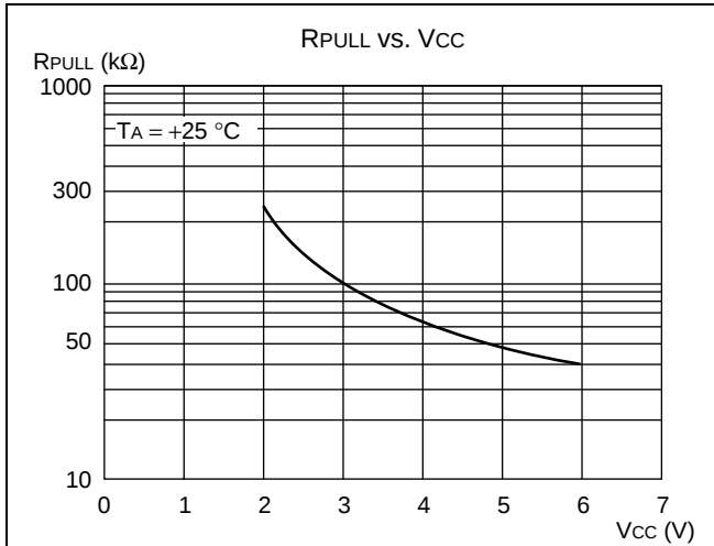
(5) Pull-up Resistance
