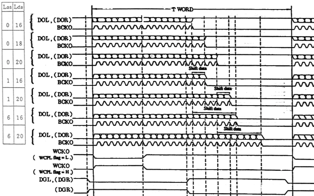
Figure C Unit output word timing (when \overline{CKSL} = L ) Lda: Number of DAC bits Las: Number of analog shift bits
