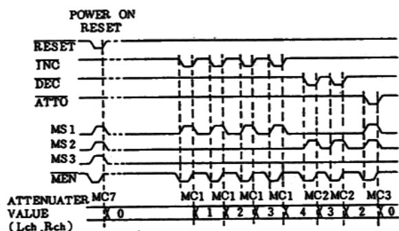
Figure 9 (Figure 8) Operation timing
