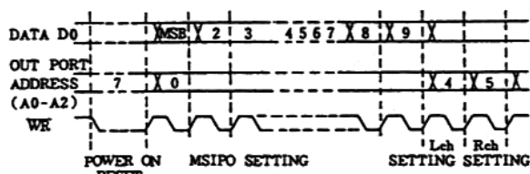
Figure 11 Operation timing of (Figure 10)
