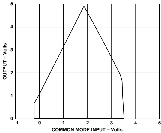
Figure 22. Maximum Output Voltage vs. Common Mode, G \geq 10 , V_S = +5 V , R_L = 100 \text{ k}\Omega
