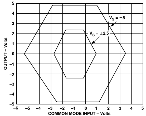
Figure 19. Maximum Output Voltage vs. Common Mode, G = 1 , R_L = 100 k\Omega
