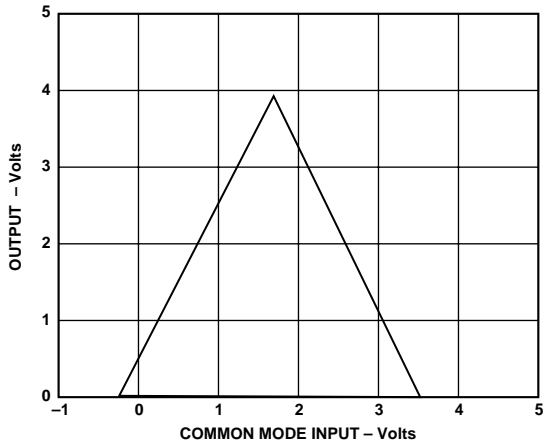
Figure 21. Maximum Output Voltage vs. Common Mode, G = 1 , V_S = +5 V , R_L = 100 \text{ k}\Omega
