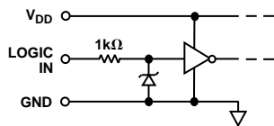
Figure 28. Equivalent Digital Input ESD Protection
