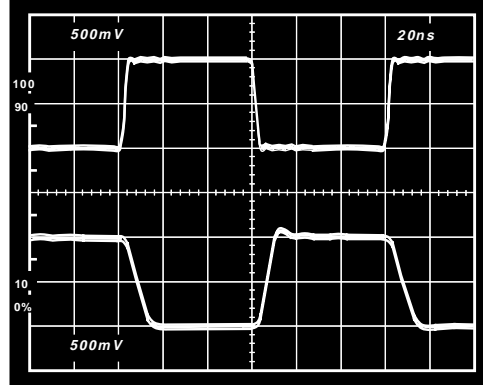
Figure 37. Small Signal Pulse Response, Gain = -1, ( R_F = 750 \Omega , R_L = 150 \Omega , V_S = \pm 5 V )
