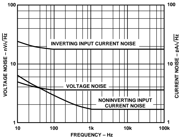
Figure 16. Input Current and Voltage Noise vs. Frequency
