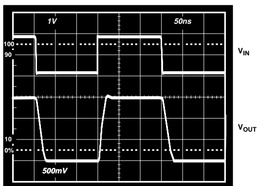
Figure 54. Pulse Response for the Circuit of Figure 52 with +V_S = 5\text{ V}
