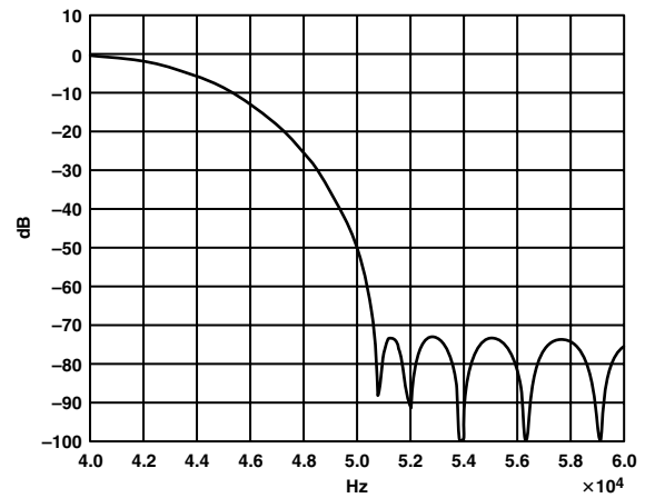
TPC 6. Transition Band Response, 4x Mode
