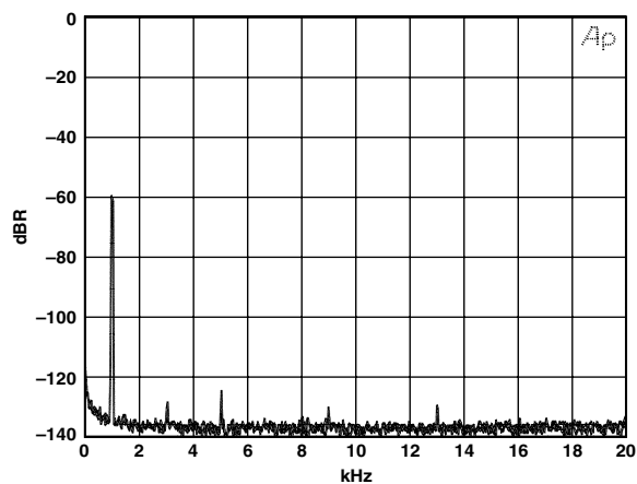
Figure 12. Dynamic Range for 1 kHz @ -60 dBFS, 110 dB, Triangular Dithered Input
