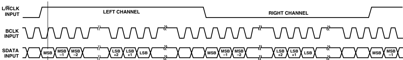
Figure 5. Left-Justified Timing Diagram
