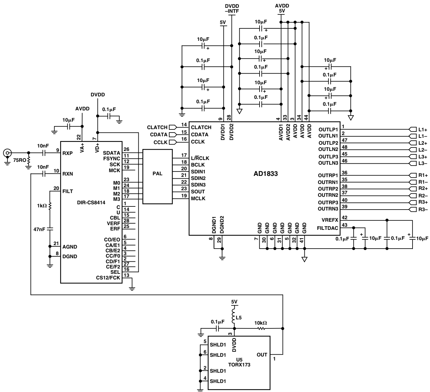
Figure 19. Example Digital Interface
