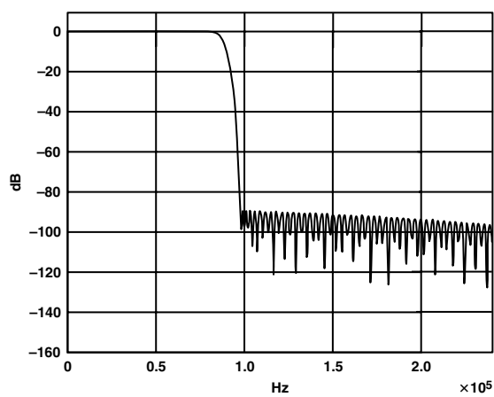
TPC 10. Complete Response, 2x Mode
