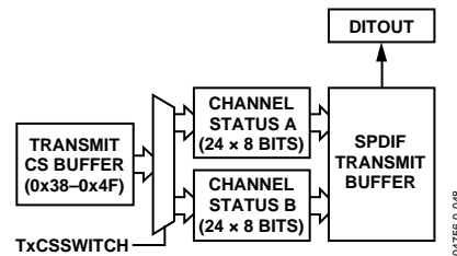
Figure 48. Transmitter Channel Status Buffer
