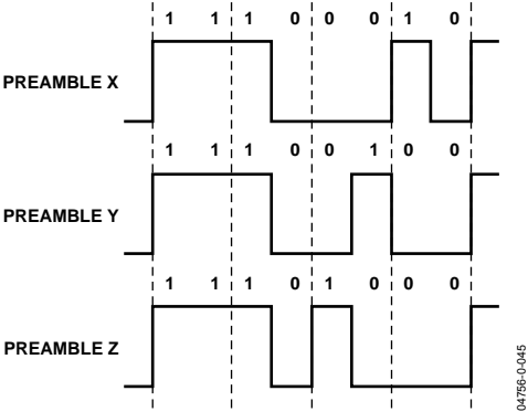
Figure 45. Preambles
