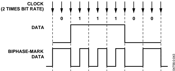
Figure 43. Biphasemark Encoding
