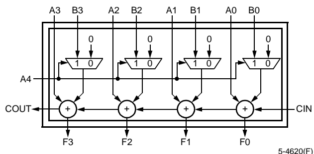
Figure 11. Multiplier Submode
