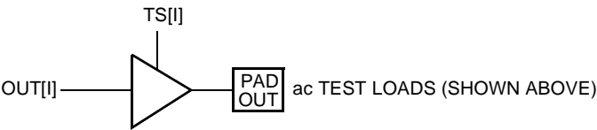
Figure 74. ac Test Loads
