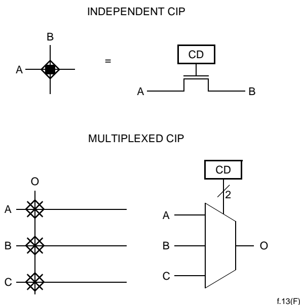
Figure 19. Configurable Interconnect Point
