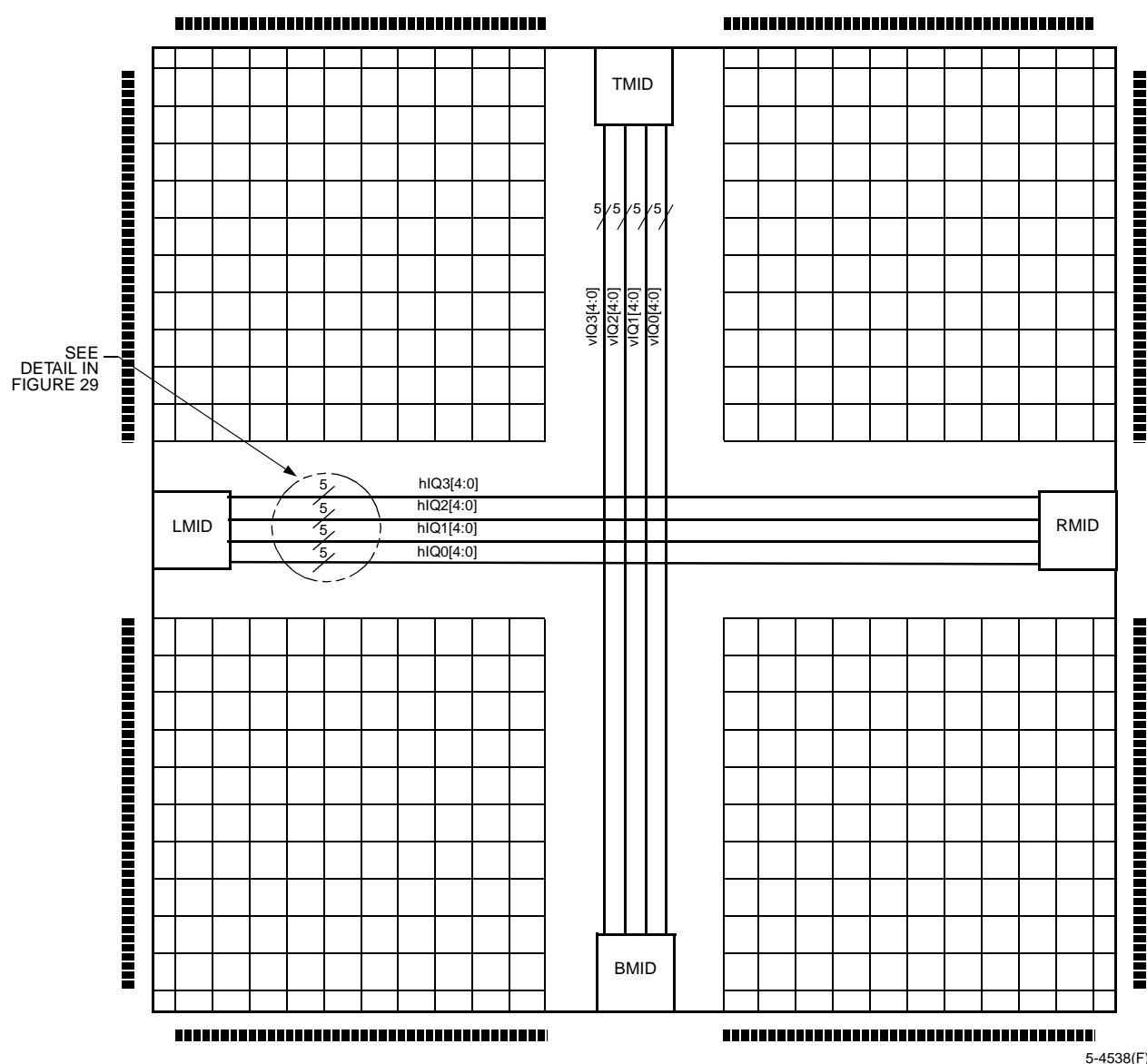
Figure 28. Interquad Routing
