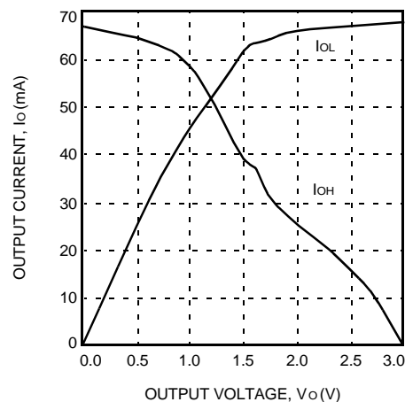
Figure 88. Fast ( T_J = 125^\circ\text{C} , V_{DD} = 3.0\text{ V} )
