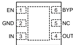
MIC5255-x.xBML 6-Pin 2mm × 2mm MLF™ (ML) (Top View)
