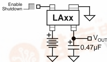
SOT-143 Version
