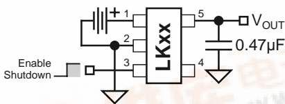
SOT-23-5 Version
