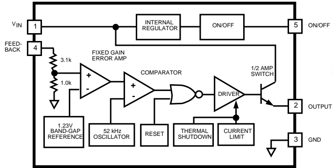
Fixed Regulator
