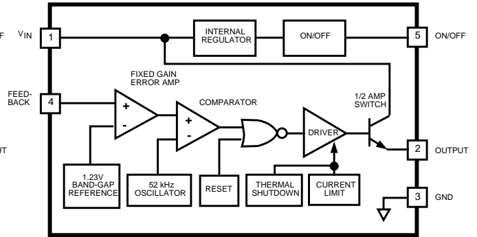
Adjustable Regulator
