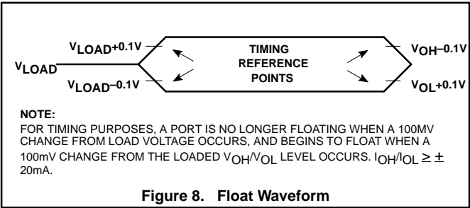
Figure 8. Float Waveform
