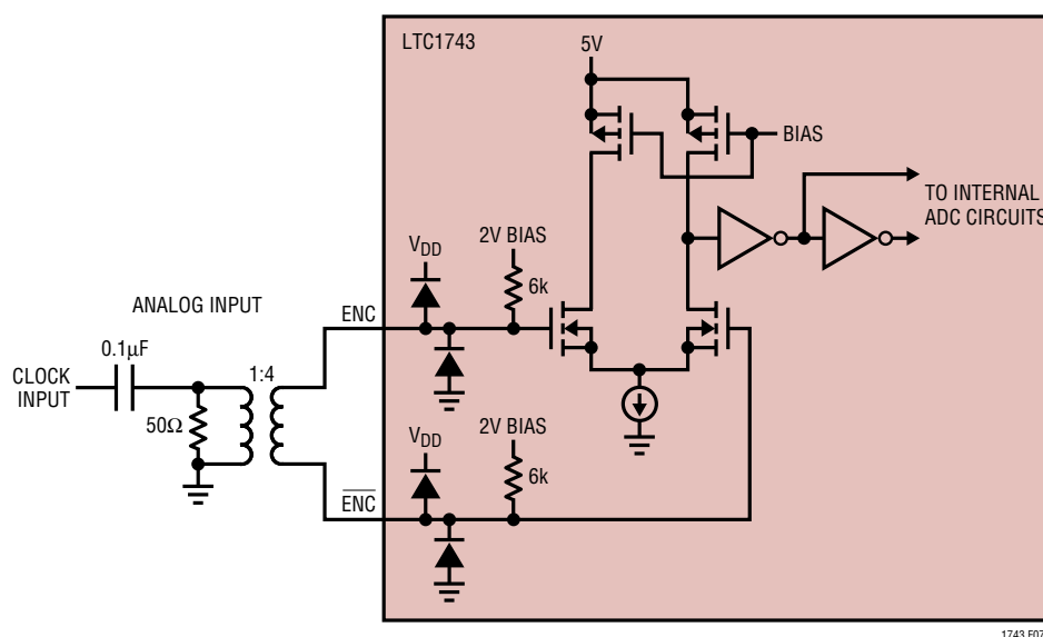
Figure 7. Transformer Driven ENC/\overline{ENC} with Equivalent Encode Input Circuit
