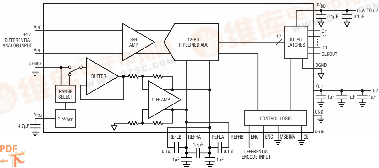
50Msps, 12-Bit ADC with a 2V Differential Input Range
