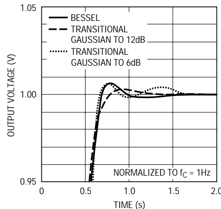
Figure 4c. Step Response—Settling
