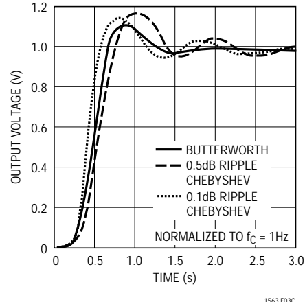
Figure 3c. Step Response
