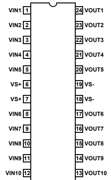
EL5323 (24-PIN TSSOP) TOP VIEW
