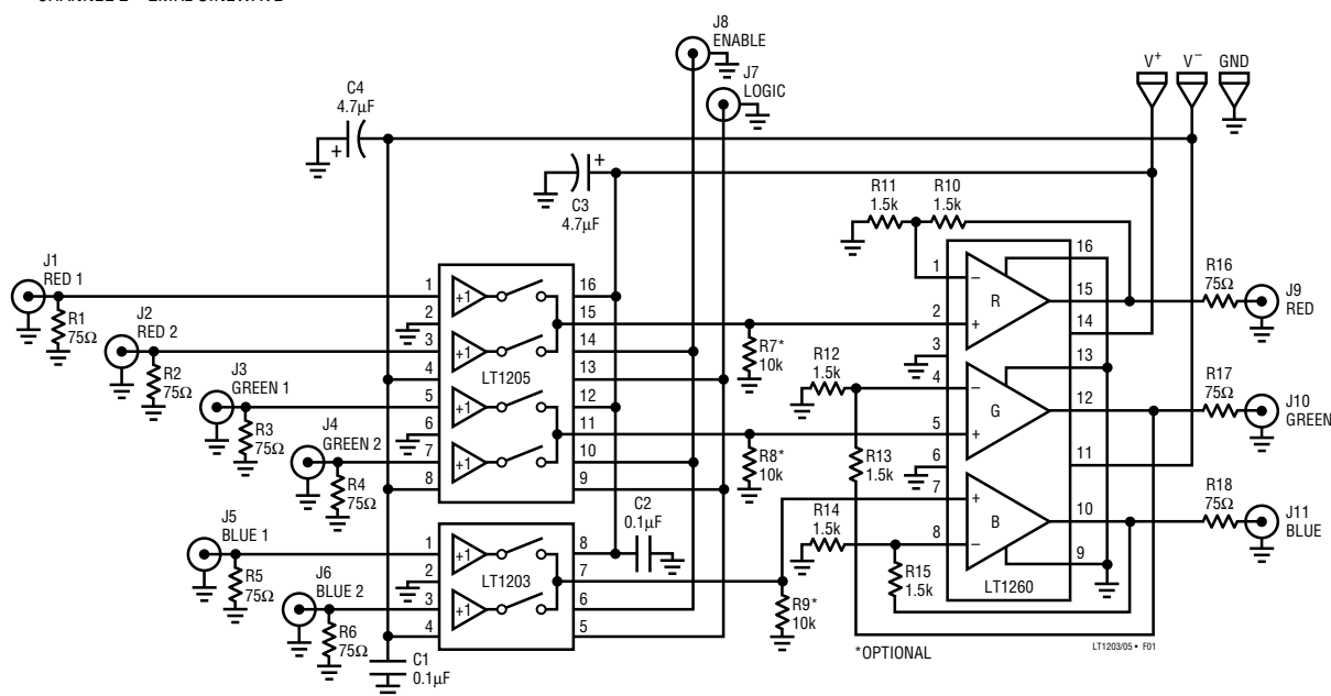
Figure 1. RGB MUX
