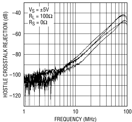
4 × 4 Crosspoint, All Hostile Rejection
