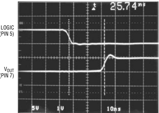
VIN1 to VIN0 Select Time
