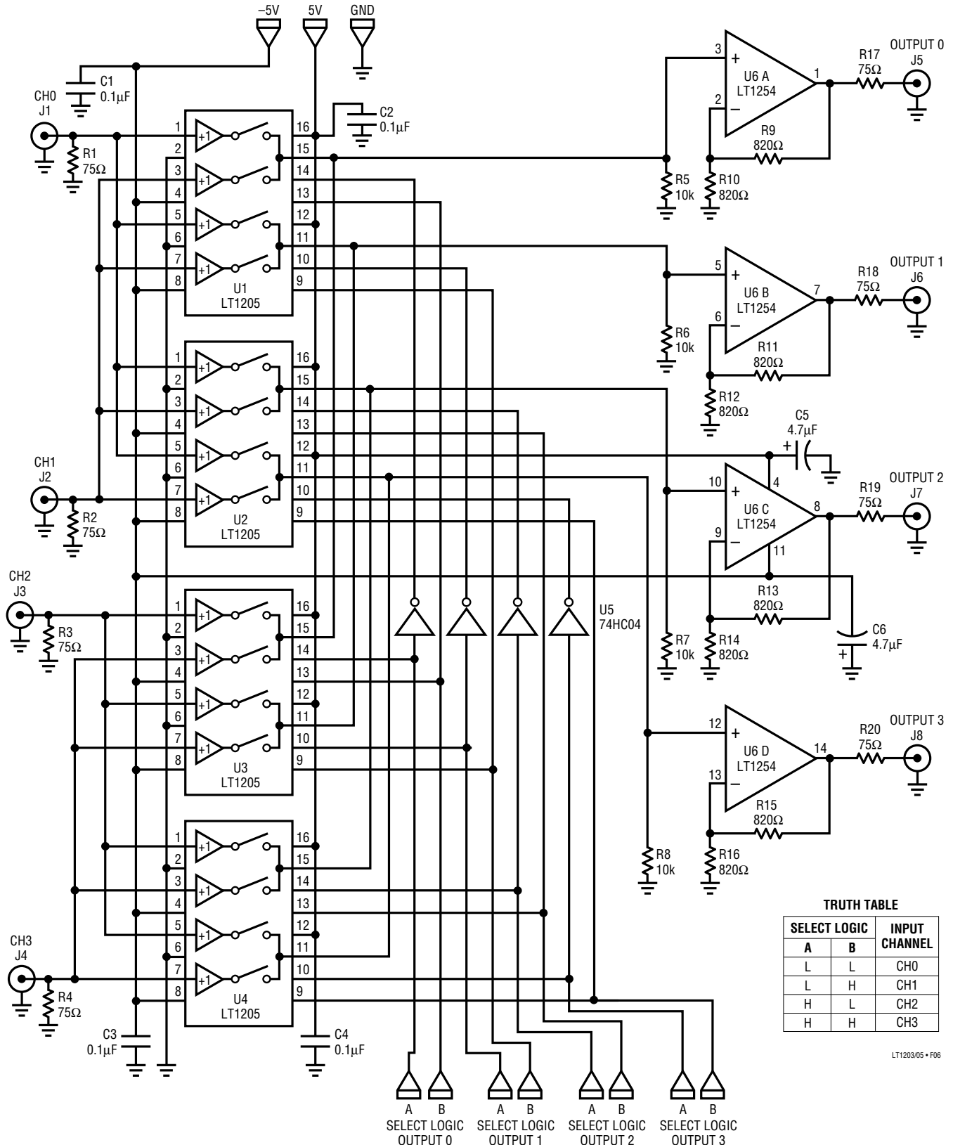
Figure 6. 4 \times 4 Crosspoint and Truth Table
