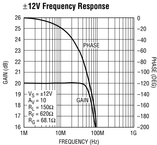
LT1253/54 • TPC14
