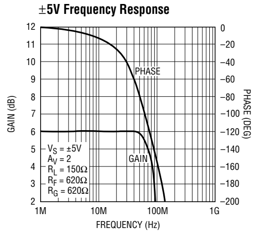
LT1253/54 • TPC13
