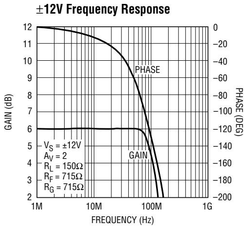
LT1253/54 • TPC12
