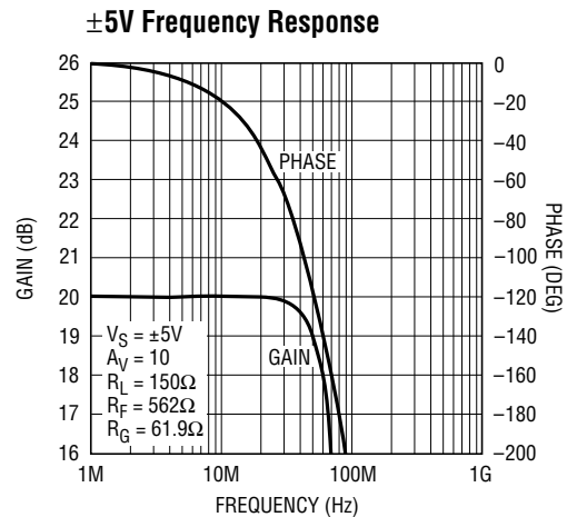
LT1253/54 • TPC15
