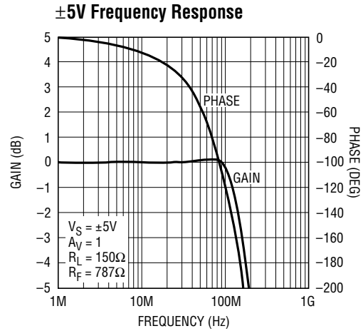
LT1253/54 • TPC11
