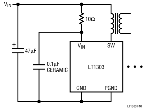
Figure 10. 10\Omega - 1\mu F Network to LT1303 V_{IN} Pin Provides Additional Decoupling. Recommended When Driving Transformers.
