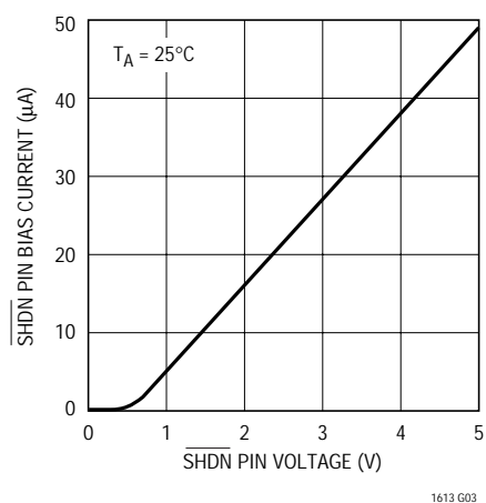
\overline{\text{SHDN}} Pin Current vs V_{\overline{\text{SHDN}}}
