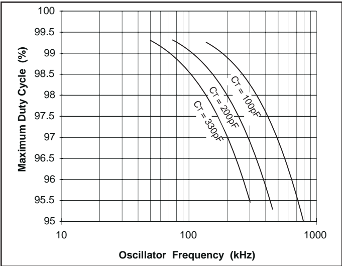
Figure 4. UCC3813-0/-2/-3 max. duty cycle vs.
