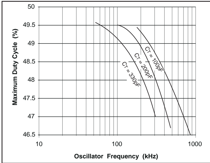
Figure 7. UCC3813-1/-4/-5 max. duty cycle vs.
