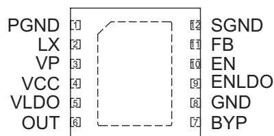
TDFN33-12 (TopView)
