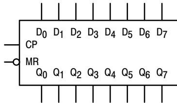
Figure 2. Logic Symbol
