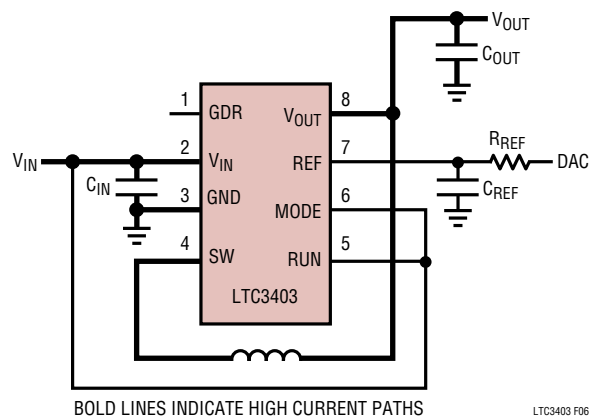
Figure 6. Layout Diagram
