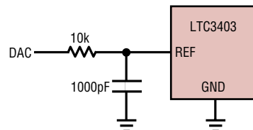
Figure 3. Filtering the REF Pin
