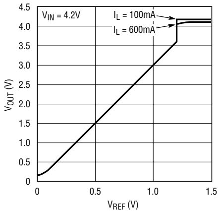
V OUT vs V REF
