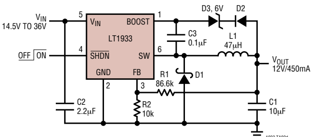
12V Step-Down Converter
