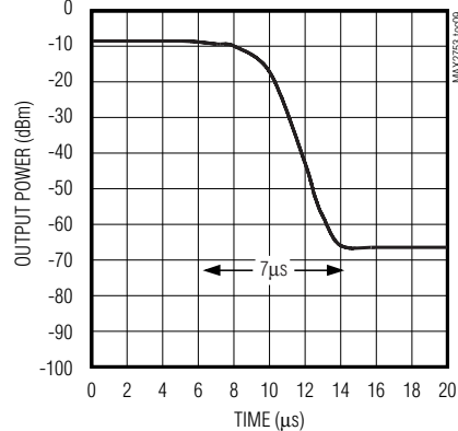
OSCILLATOR TURN-OFF TIME
