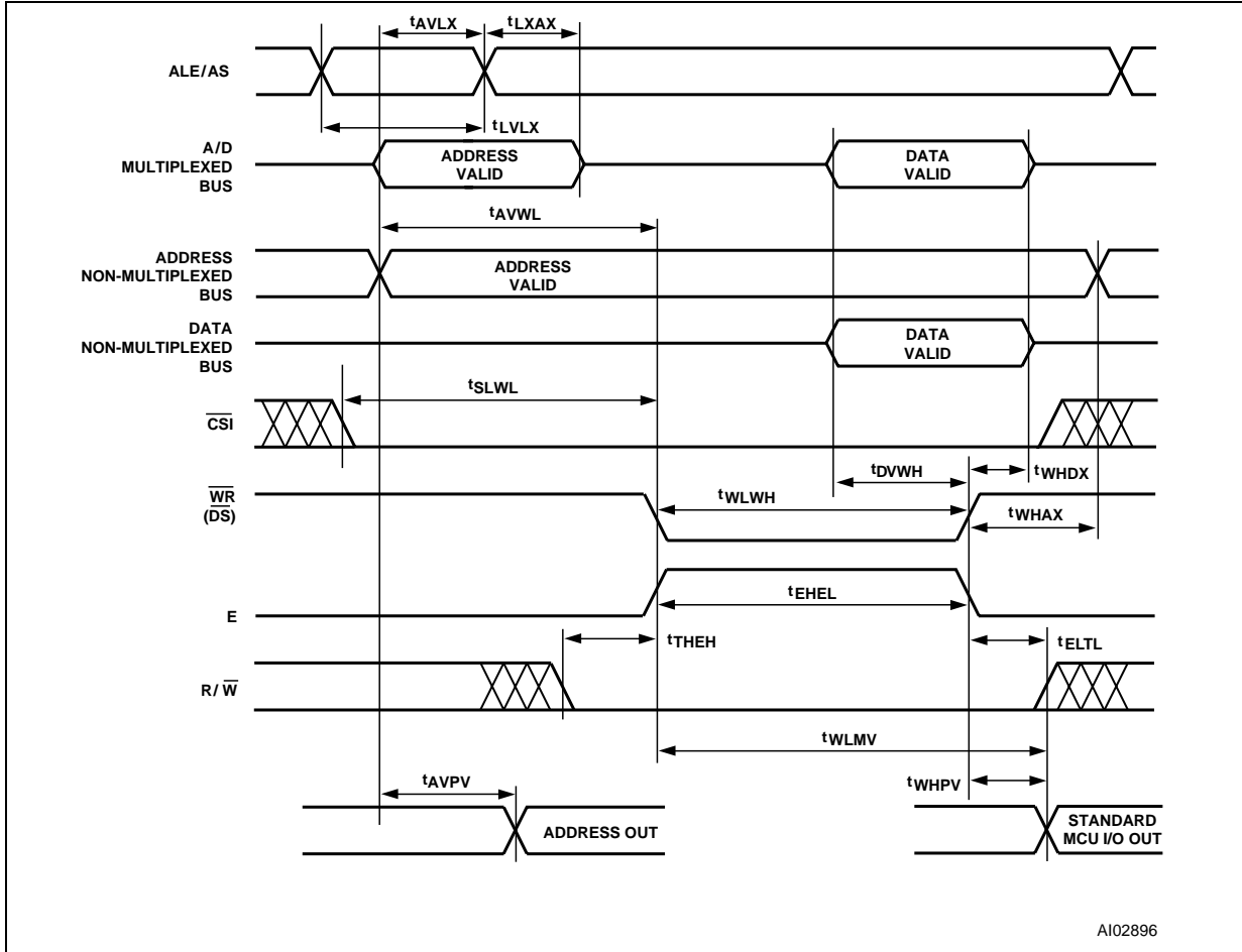
Figure 48. WRITE Timing
