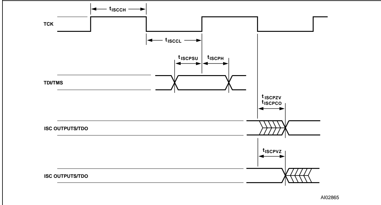
Figure 52. ISC Timing
