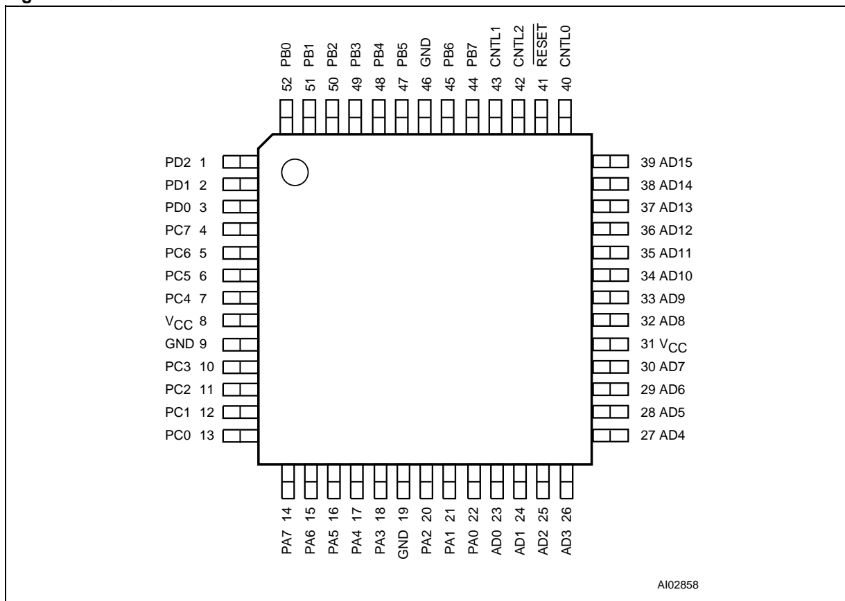
Figure 2. PQFP52 Connections
