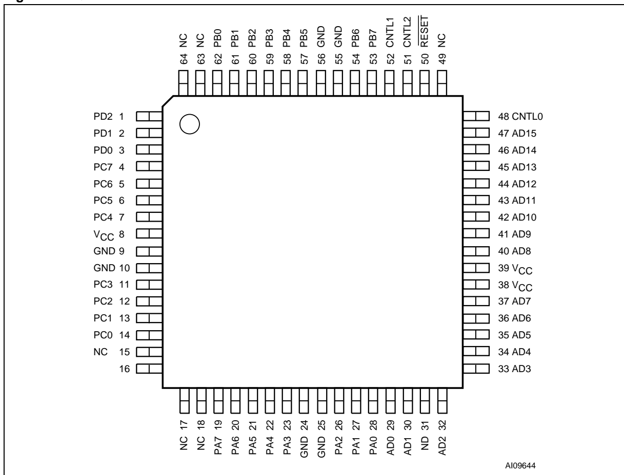
Figure 4. TQFP64 Connections
