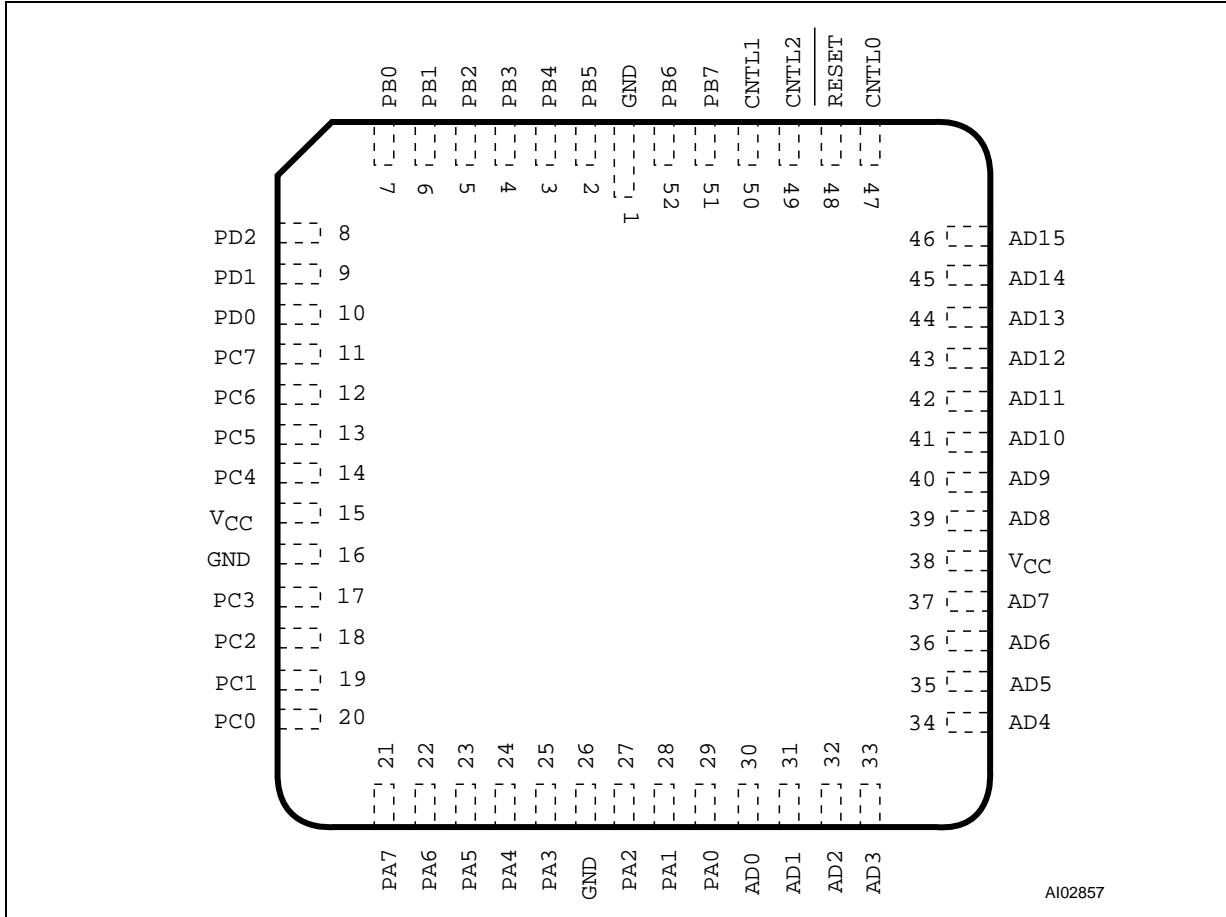
Figure 3. PLCC52 Connections
