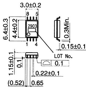
BA2903FV(SSOP-B8) (Unit:[mm])
