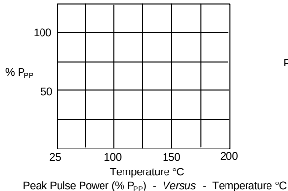
Figure 2 - Derating Curve
