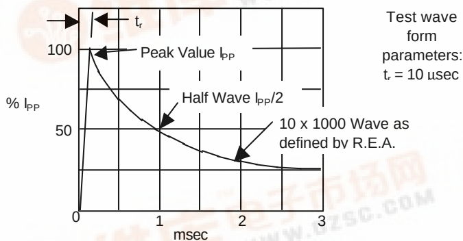
Figure 1 - Pulse Waveform
