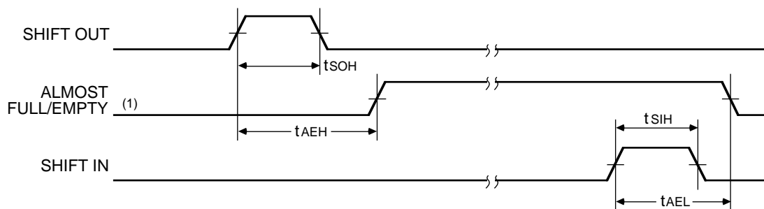
Figure 9. t_{AEH} and t_{AEL} Specifications
