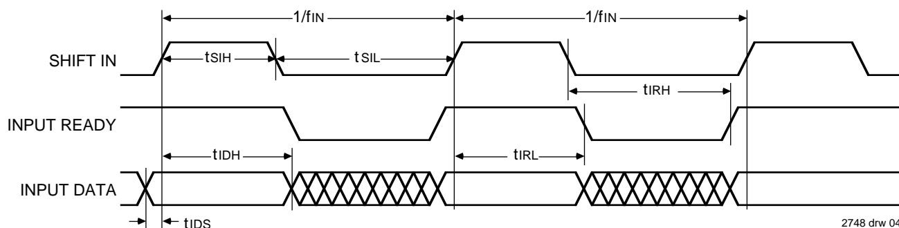
Figure 2. Input Timing
