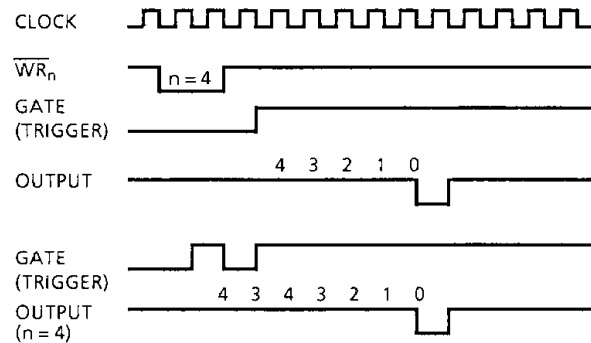
Figure 6.1 TMP8253 Timing Diagrams
