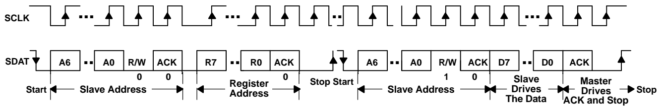
Figure 43. Serial Interface READ From TPS65013: Protocol B
