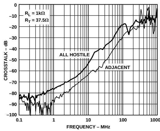
Figure 15. AD8115 Crosstalk vs. Frequency
