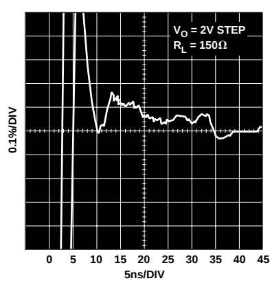
Figure 17. AD8115 Settling Time
