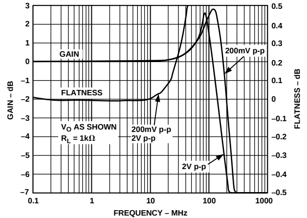
Figure 10. AD8115 Frequency Response; R_L = 1 k\Omega
