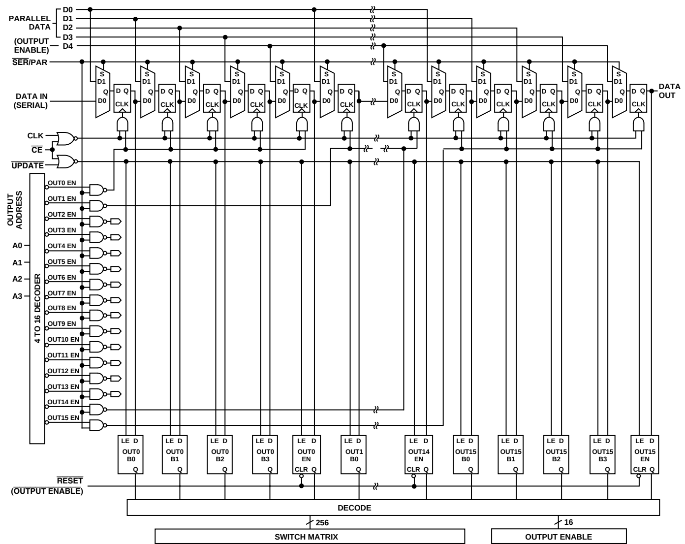
Figure 4. Logic Diagram
