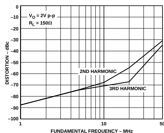
Figure 16. AD8115 Distortion vs. Frequency
