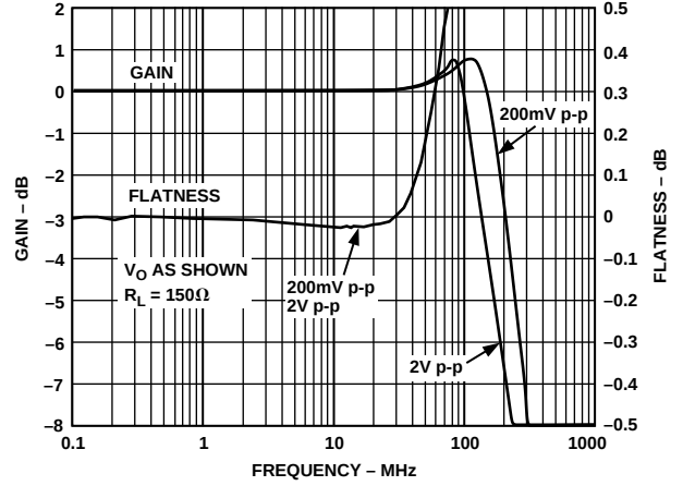
Figure 9. AD8115 Frequency Response; R_L = 150 \Omega
