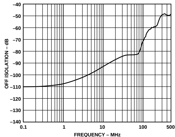
Figure 27. AD8115 Off Isolation, Input-Output
