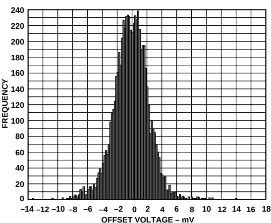
Figure 40. AD8115 Offset Voltage Distribution
