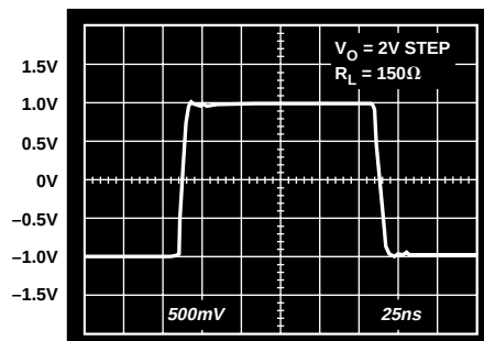
Figure 31. AD8114 Pulse Response, Large Signal
