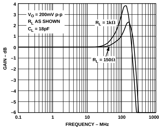
Figure 8. AD8114 Frequency Response vs. Load Impedance
