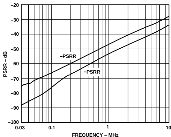
Figure 25. AD8114 PSRR vs. Frequency
