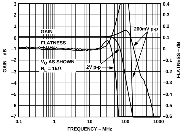
Figure 7. AD8114 Frequency Response; R_L = 1 k\Omega
