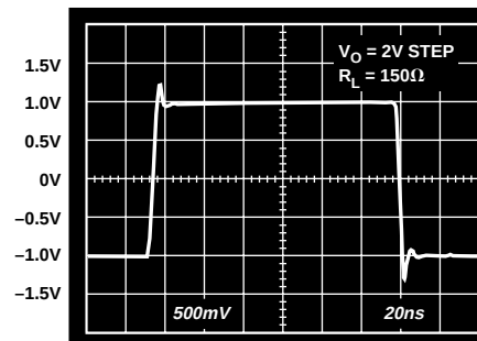
Figure 34. AD8115 Pulse Response, Large Signal
