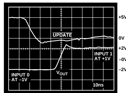
Figure 35. AD8115 Switching Time
