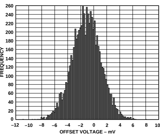
Figure 37. AD8114 Offset Voltage Distribution
