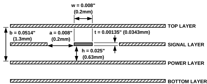
Figure 51. Cross Section of Input and Output Traces
