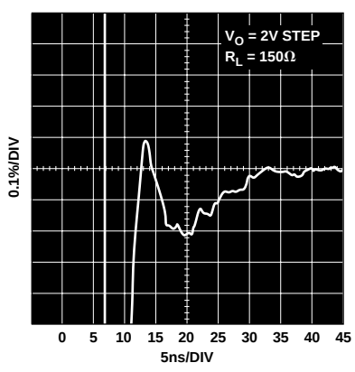
Figure 14. AD8114 Settling Time
