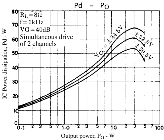
Figure 1. STK4171V Pd - P_O ( R_L = 8\Omega )
