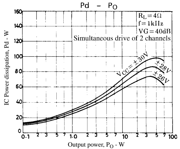
Figure 2. STK4171V Pd - P_O ( R_L = 4\Omega )
