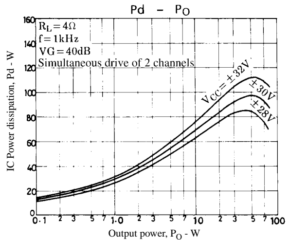
Figure 2. STK4181V Pd - P O ( R_L = 4\Omega )
