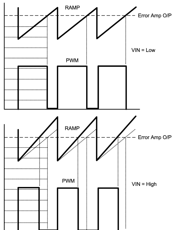
FIGURE 1. Voltage Feedforward
