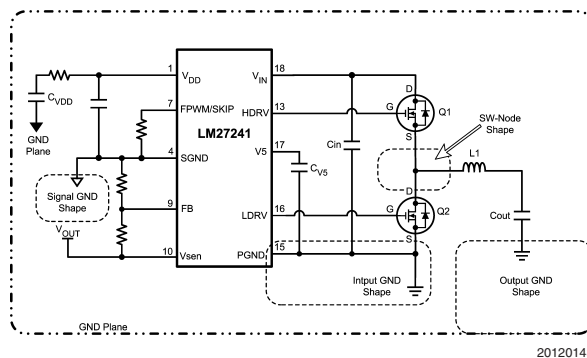
FIGURE 15. Critical Component placement (TSSOP)
