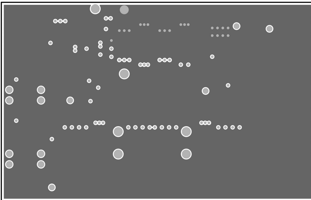
FIGURE 21. Internal Plane 2
