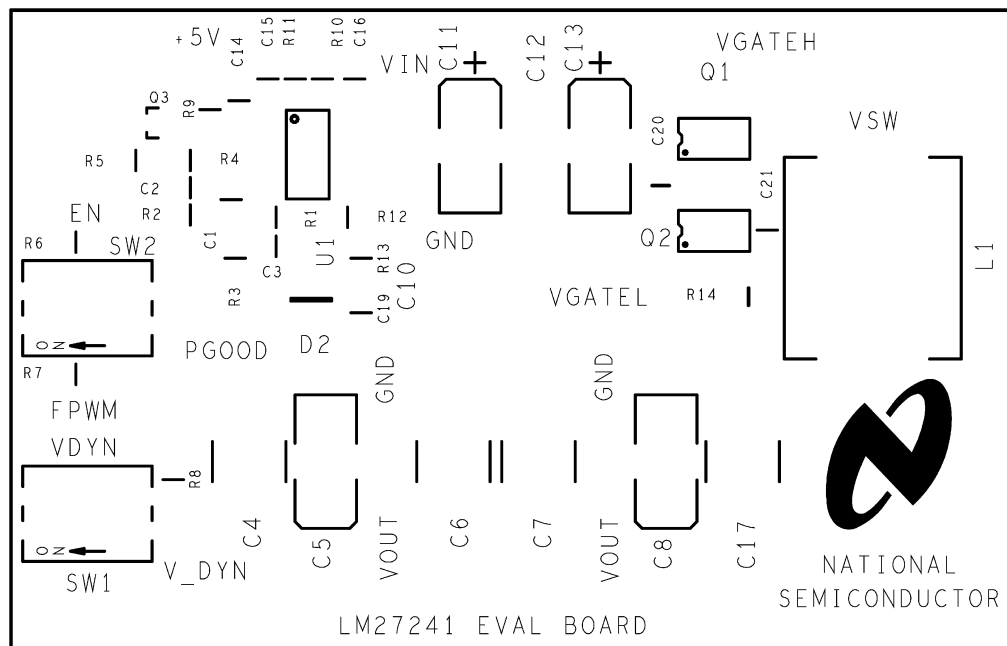
FIGURE 18. Top Overlay
