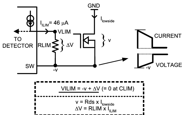
FIGURE 12. Understanding Current Sensing
