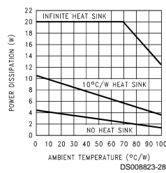
Maximum Power Dissipation (TO-3)
