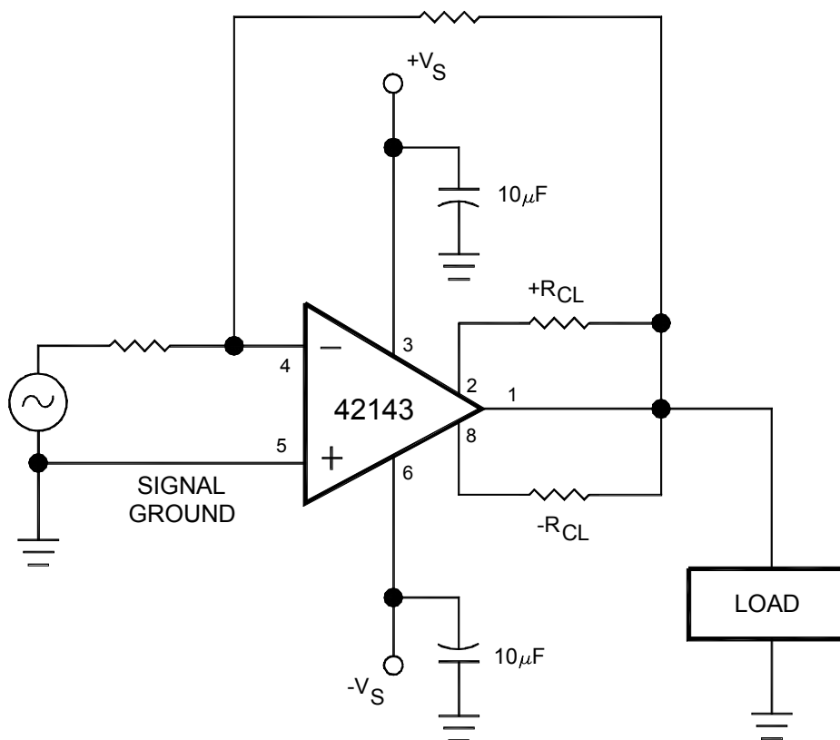
Figure 4. Application Information
