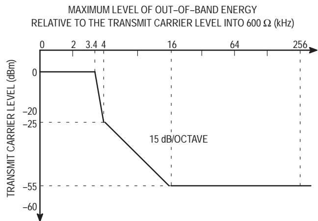
Figure 2. Out-of-Band Energy
