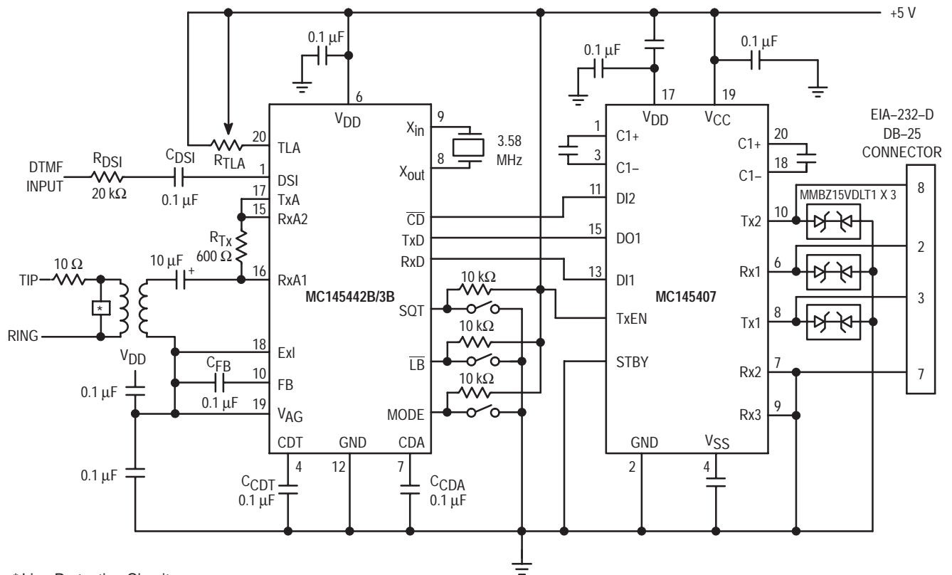
Figure 7. Typical MC145442B/MC145443B Applications Circuit
