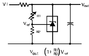
FIGURE 1. SHUNT REGULATOR
