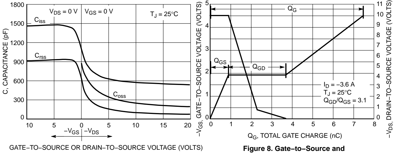
Figure 7. Capacitance Variation
