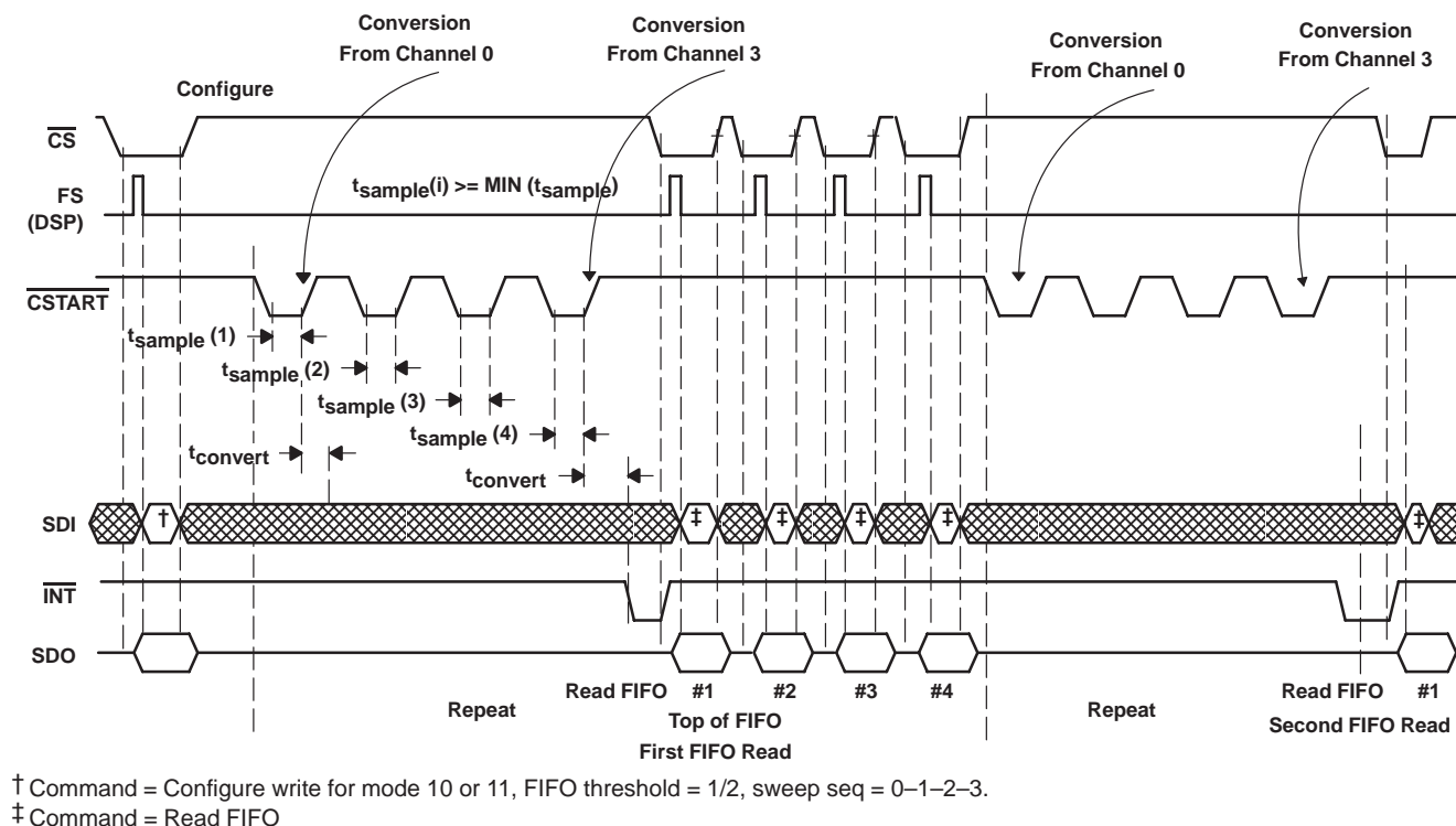
Figure 13. TLV2544/TLV2548 Mode 10/11 DSP Serial Interface (Conversions triggered by \overline{\text{CSTART}} )
