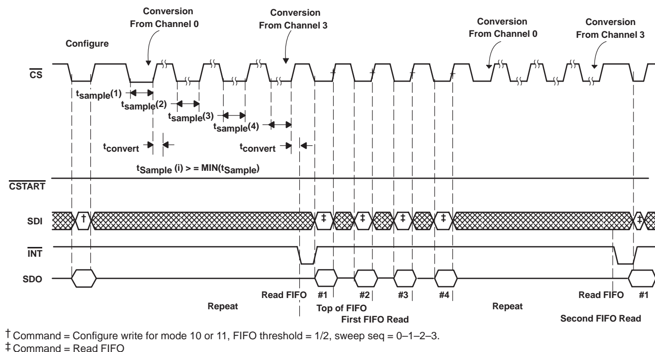
Figure 14. TLV2544/TLV2548 Mode 00/11 \mu p Serial Interface (Conversions triggered by \overline{\text{CS}} )
