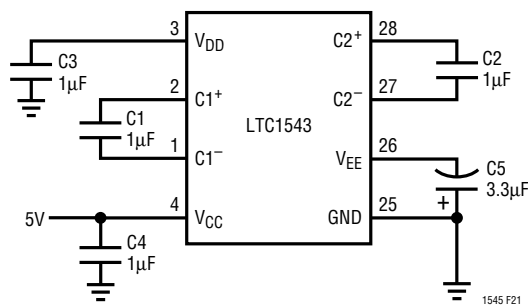
Figure 21. Charge Pump
