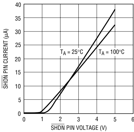
Boost Switching Regulator \overline{\text{SHDN}} Pin Current vs Voltage
