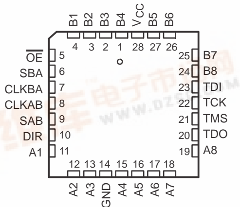
SN54ABT8646 . . . FK PACKAGE (TOP VIEW)
