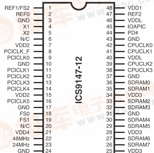
48-Pin SSOP
