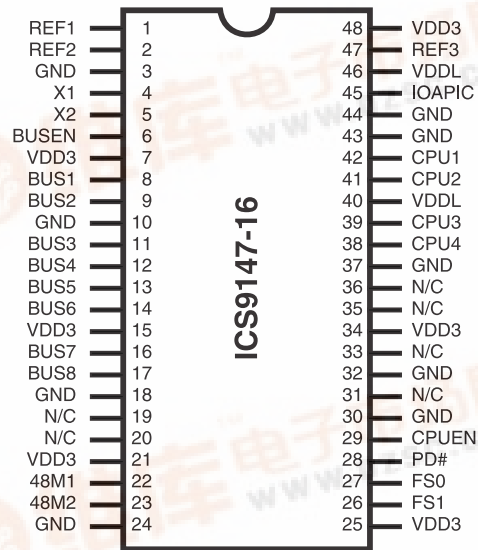
48-Pin SSOP
