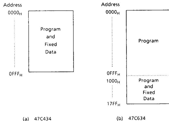
Figure 2-1. Program Memory
