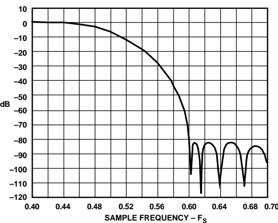
Figure 27. AD1847 Digital-to-Analog Frequency Response -Transition Band (Full-Scale Inputs, 0 dB Attenuation)
