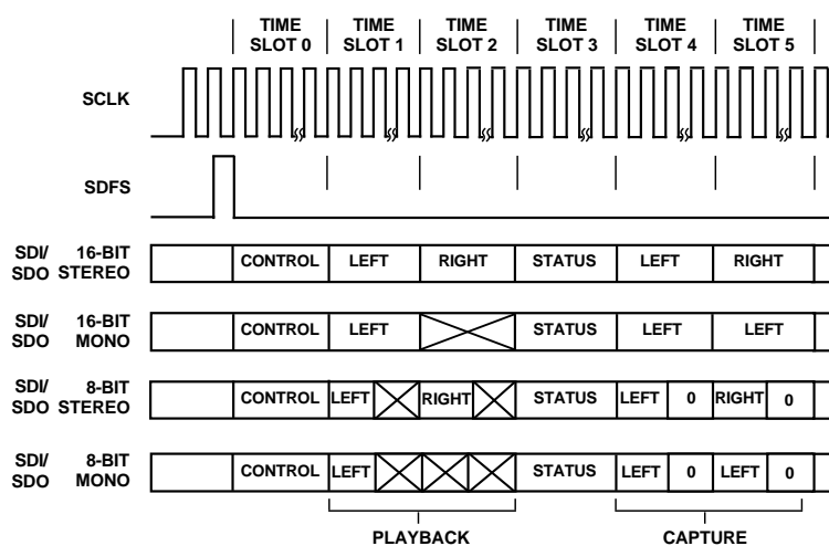
Figure 32. Serial Data Format, 1-Wire System (TSSEL = 0)
