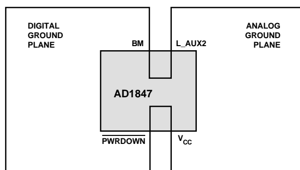
Figure 23. Recommended Ground Plane
