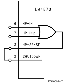
FIGURE 2. HP-SENSE Pin to SHUTDOWN Pin Connection
