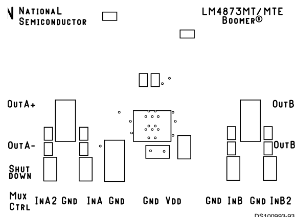
Silk Screen Layer
