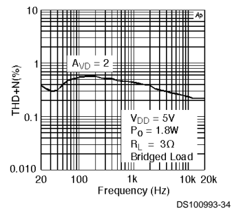
LM4873MTE THD+N vs Frequency
