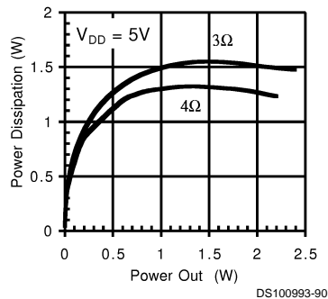
LM4873MTE Power Dissipation vs Power Output
