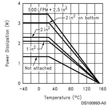
LM4873MTE-1 (Note 21) Power Derating Curve
